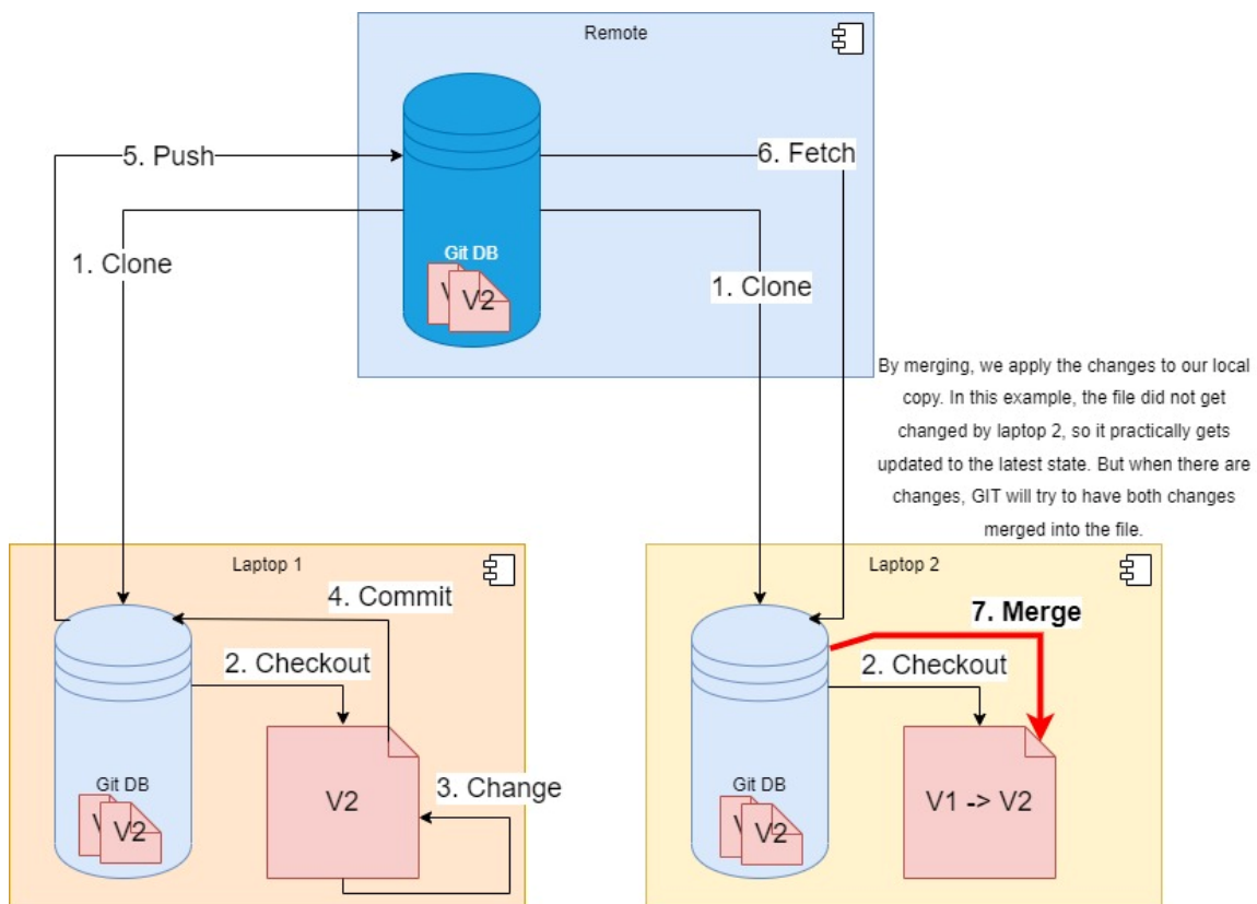
Step 7 – Merge
