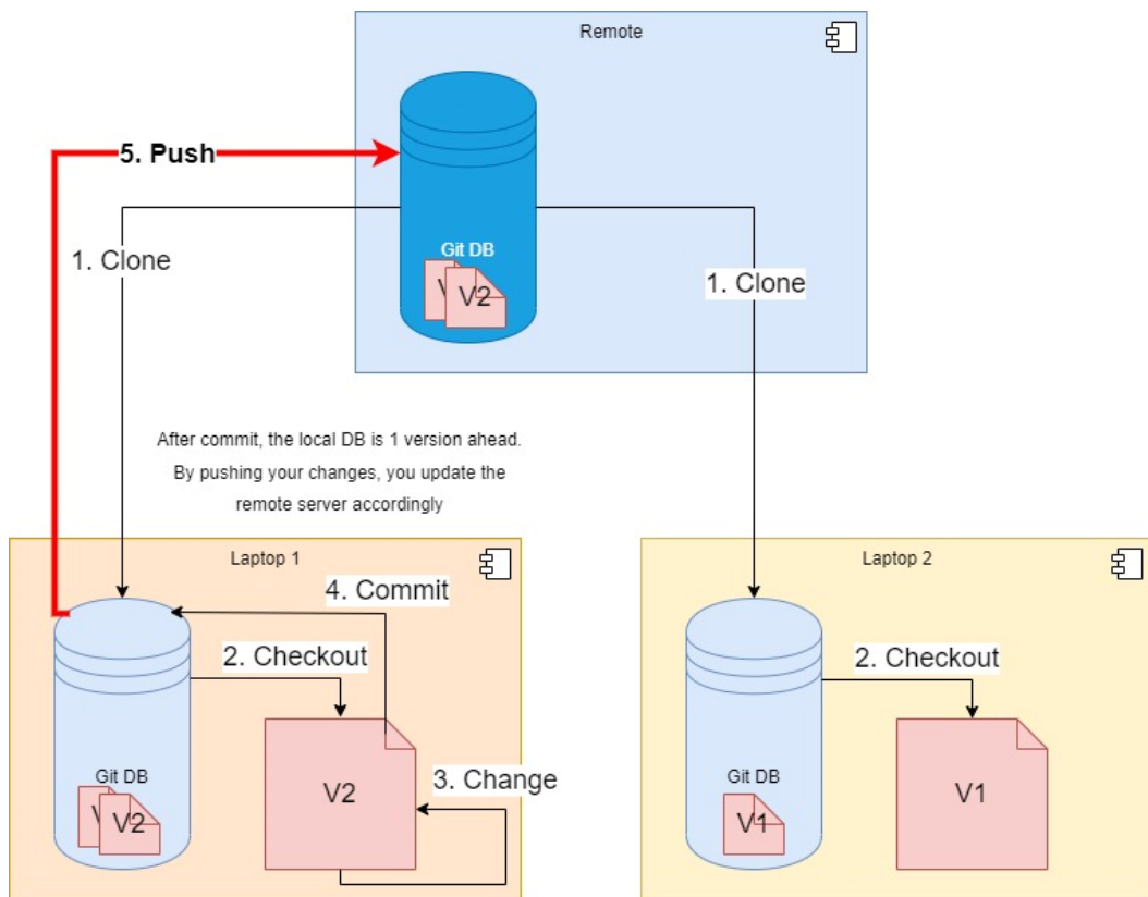
Step 5 – Push
