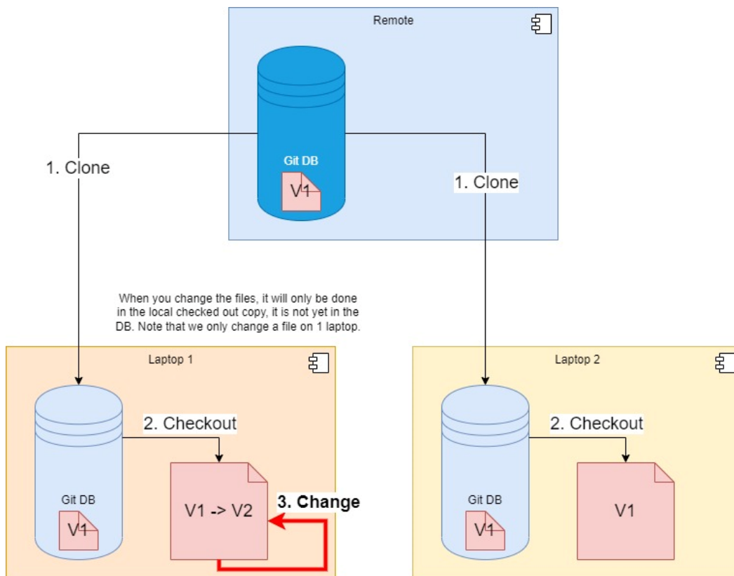
Step 3 – Change
