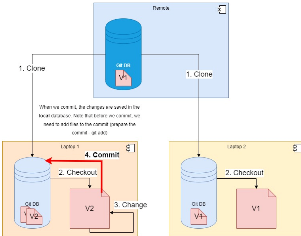
Step 4 – Commit
