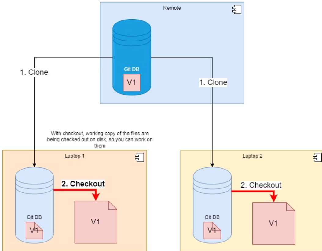
Step 2 – Checkout
