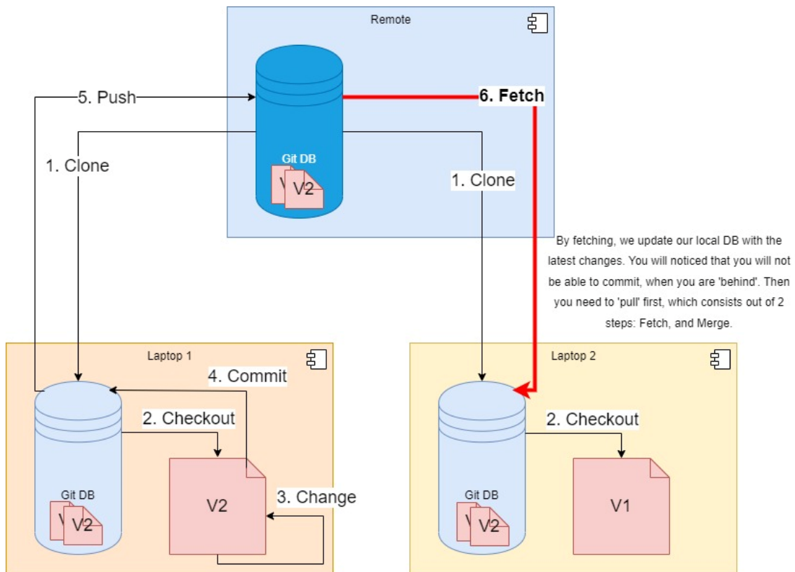
Step 6 – Fetch
